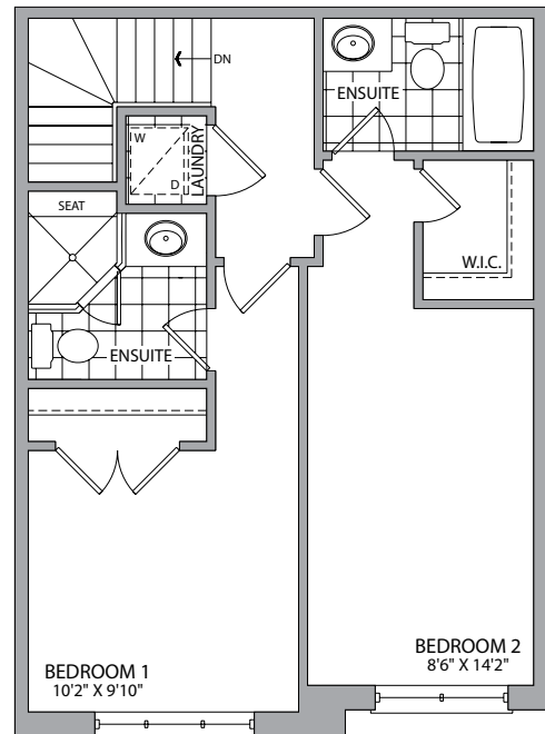
THIRD FLOOR END ELEV A BLOCK 1 - LOT 7 BLOCK 3 - LOT 19
