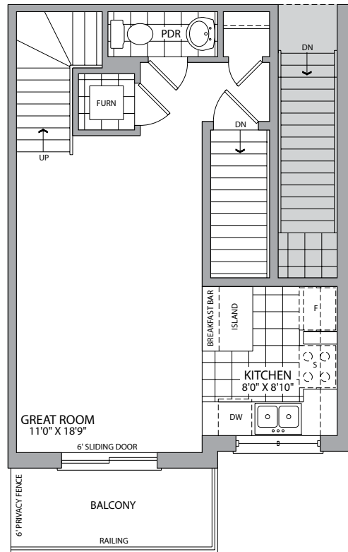
SECOND FLOOR END ELEV A BLOCK 1 - LOT 7 BLOCK 3 - LOT 19 1098 SQ. FT.
