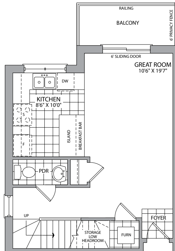
SECOND FLOOR END ELEV A, D BLOCK 1 - LOT 1 BLOCK 4 - LOT 26 1100 SQ. FT.
